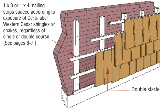
Figure 14: Over Masonry Detail
